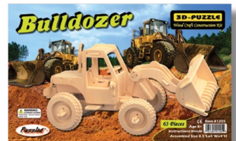
1205 Bulldozer
